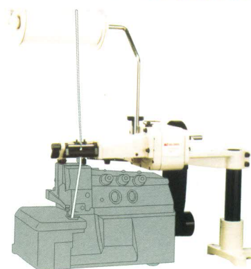
MDK 60-2 包縫車用(基座固定於車板上) FOR OVERLOCK (Base is mounted on the table)
