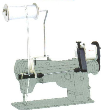
MDK 61-2 包縫車用專用型(基座固定於機頭上) FOR SPECIFIC OVERLOCK (Base is mounted on the machine head)
